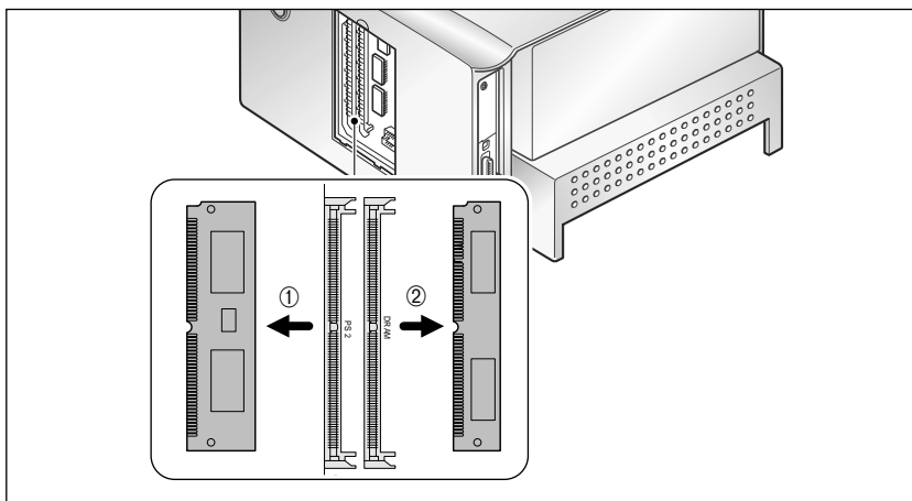
1. Remove Post Script SIMM
